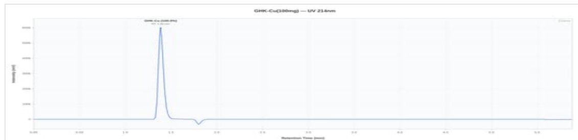
GHK-Cu 100mg - BB-GHKCU100-2601: UV Chromatogram
